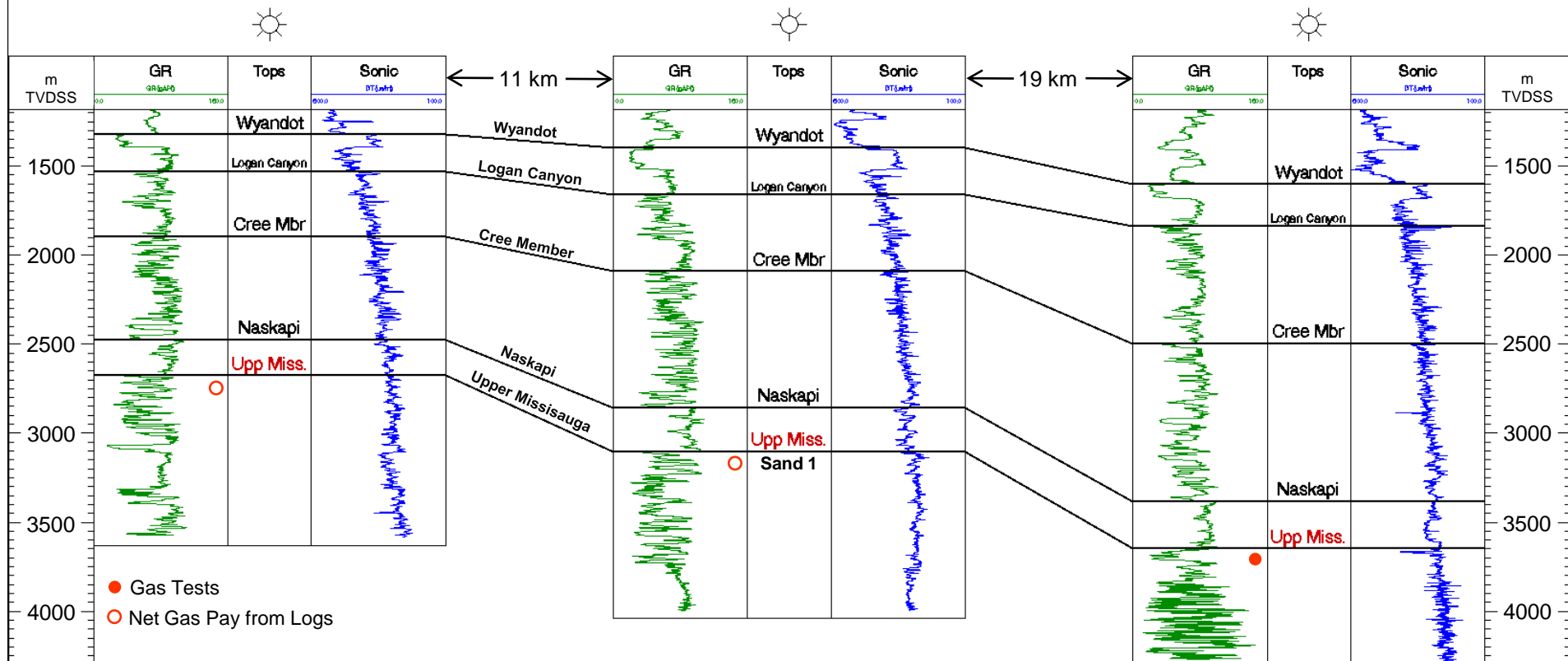
Onondaga to North Triumph Structural Cross-Section (Wyandot Fm. to TD). The main gas bearing zone, in each well, is located at the top of the Missisauga Formation directly below the Naskapi shale. The North Triumph gas field is a Commercial Discovery and is currently producing as part of the Sable Gas Project and the Onondaga gas field is a Significant Discovery. Note this xsection crosses Parcel #1 from west to east.
